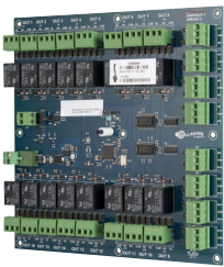
HBUS 16 In 16 Out Board C300688
